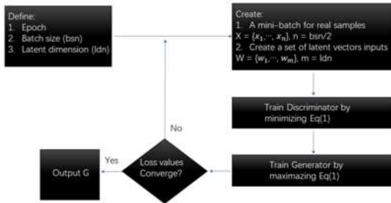
Fig. 3 Step-by-step illustration of GAN training algorithm
